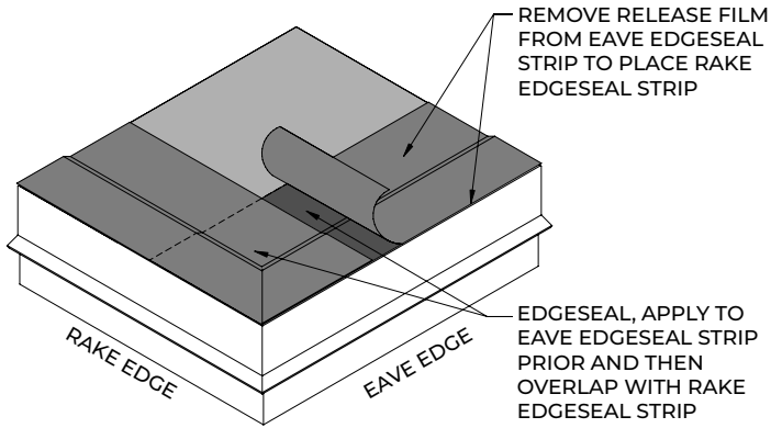
EDGESEAL INSTALLATION
