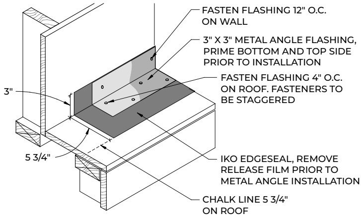
RAKE / WALL CONNECTION DETAIL
