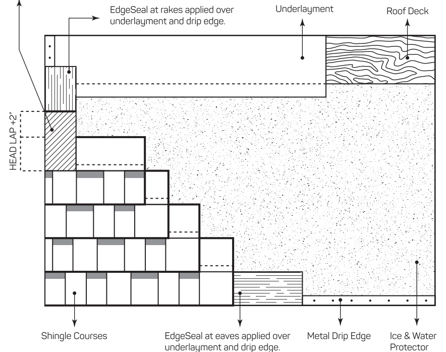
Detail B: Installation Diagram for High-Wind Regions and Miami-Dade NOA
