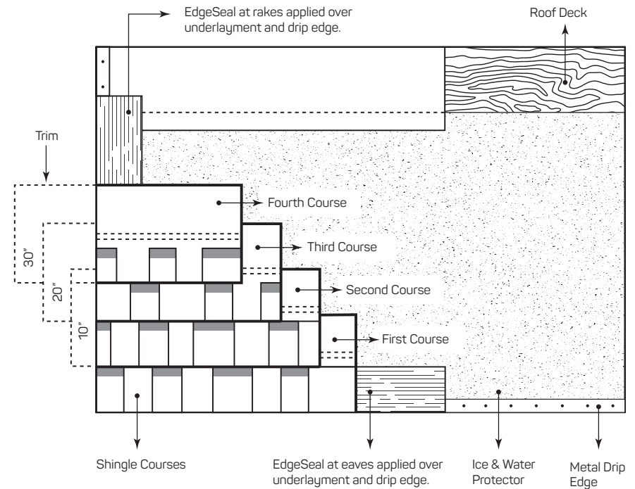
Detail G: Install the First Course
