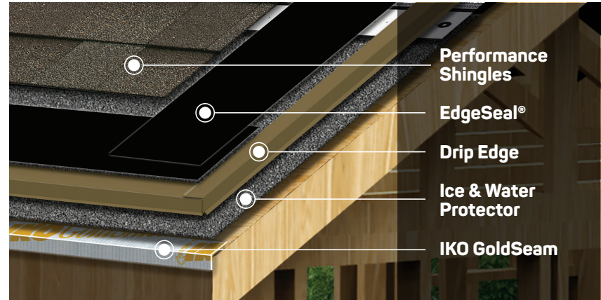
Detail A: Installation Diagram for Eaves and Rakes
