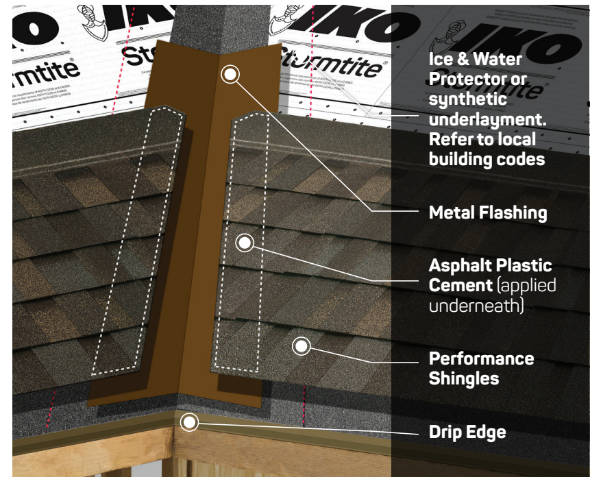
Detail D: EdgeSeal Installation Diagram for Valley
