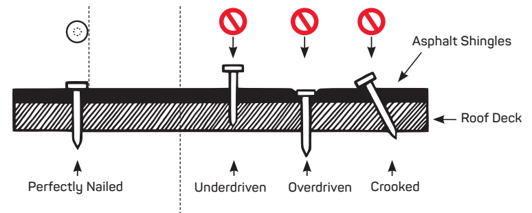
Detail C: Diagram for proper nailing on IKO Dynasty and Nordic Performance shingles
