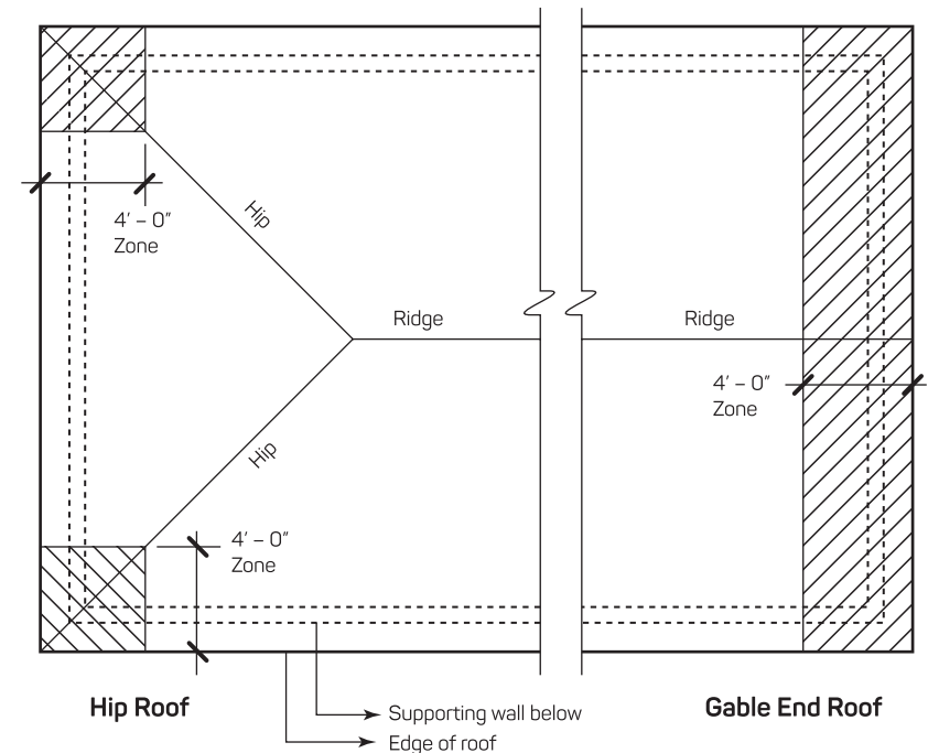
Figure 1: Typical Plan View for Roof
