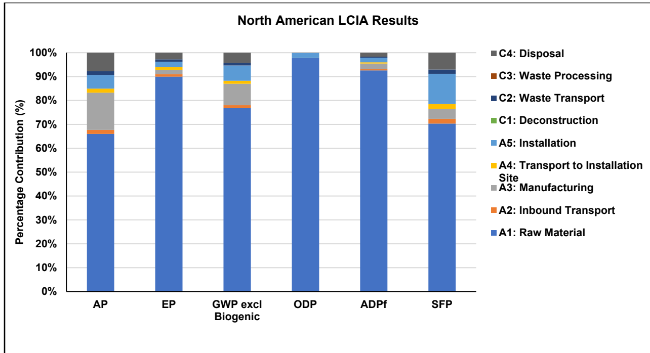
Figure 4: Contribution analysis of North American LCIA results
