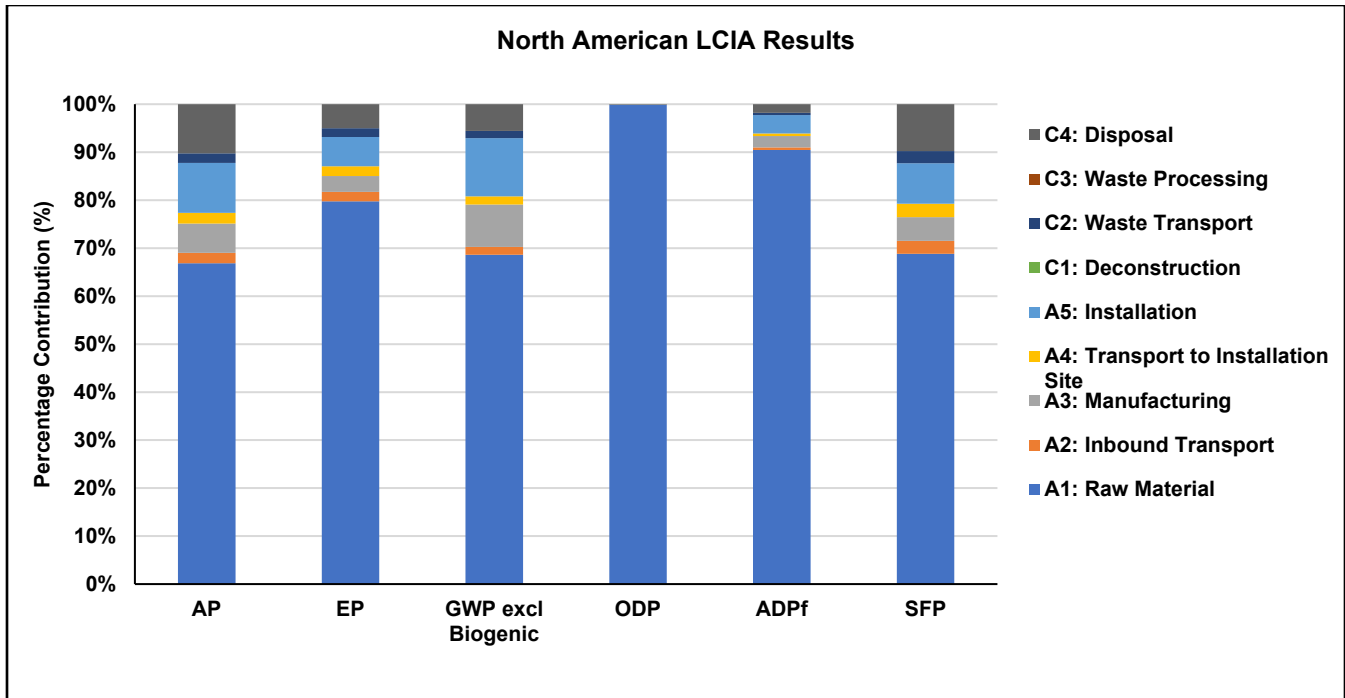
Figure 4: Contribution Analysis of North American LCIA Results
